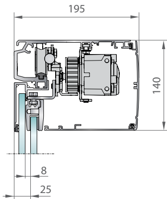
Single and bi-parting systems with side panel
