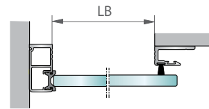
Single door leaf without side panel Wall mounting
