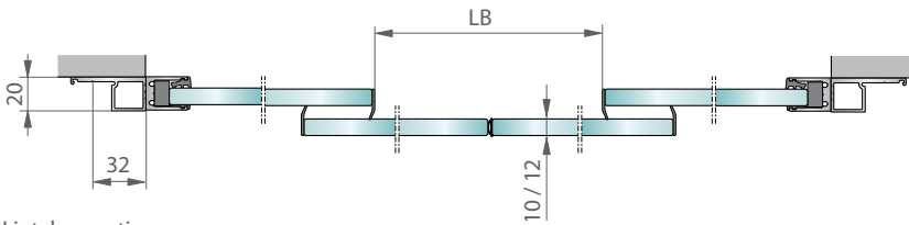
Lintel mounting
