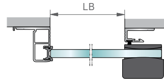
Lintel mounting
