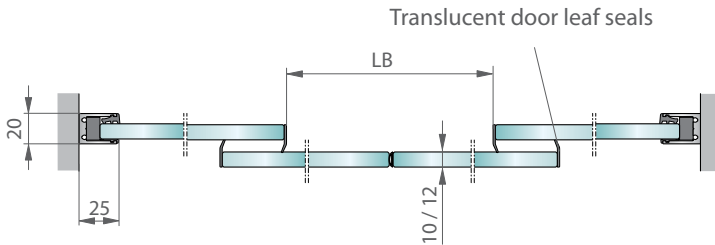
Bi-parting door with side panel Wall mounting
