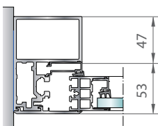
Jamb reinforced
